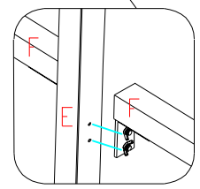
Step 9 To tear down the side eaves rail
