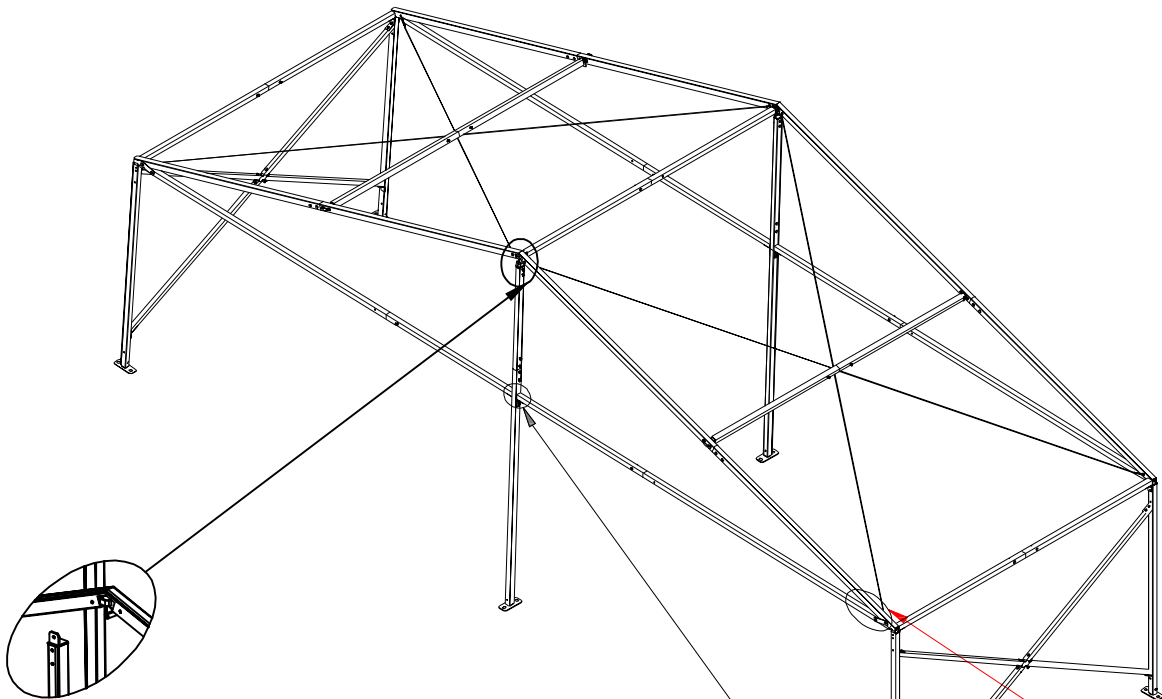
Step 10 To tear down the Gable pole
